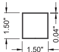
TG-T-215 TUBE ALUM. 6063-T6
