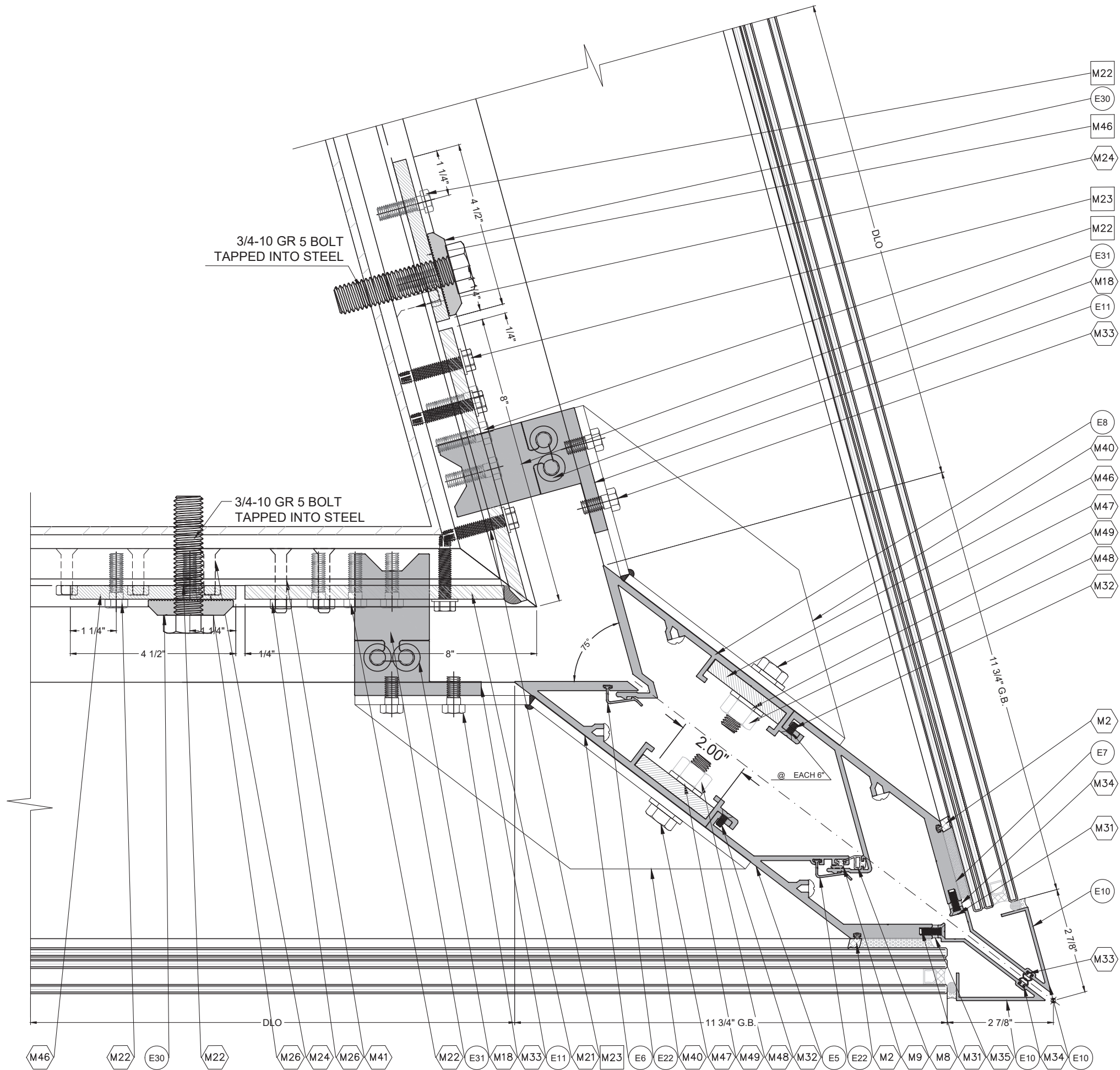
1 D4 DETAIL PARTIAL 75° CORNER
