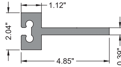
E32 GW-7000-142A MULLION ANCHOR FIST ALUM. 6061-T6
