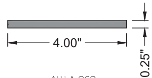
E41 ALU-A-060 SHIM PLATE ALUM. 6063-T6
