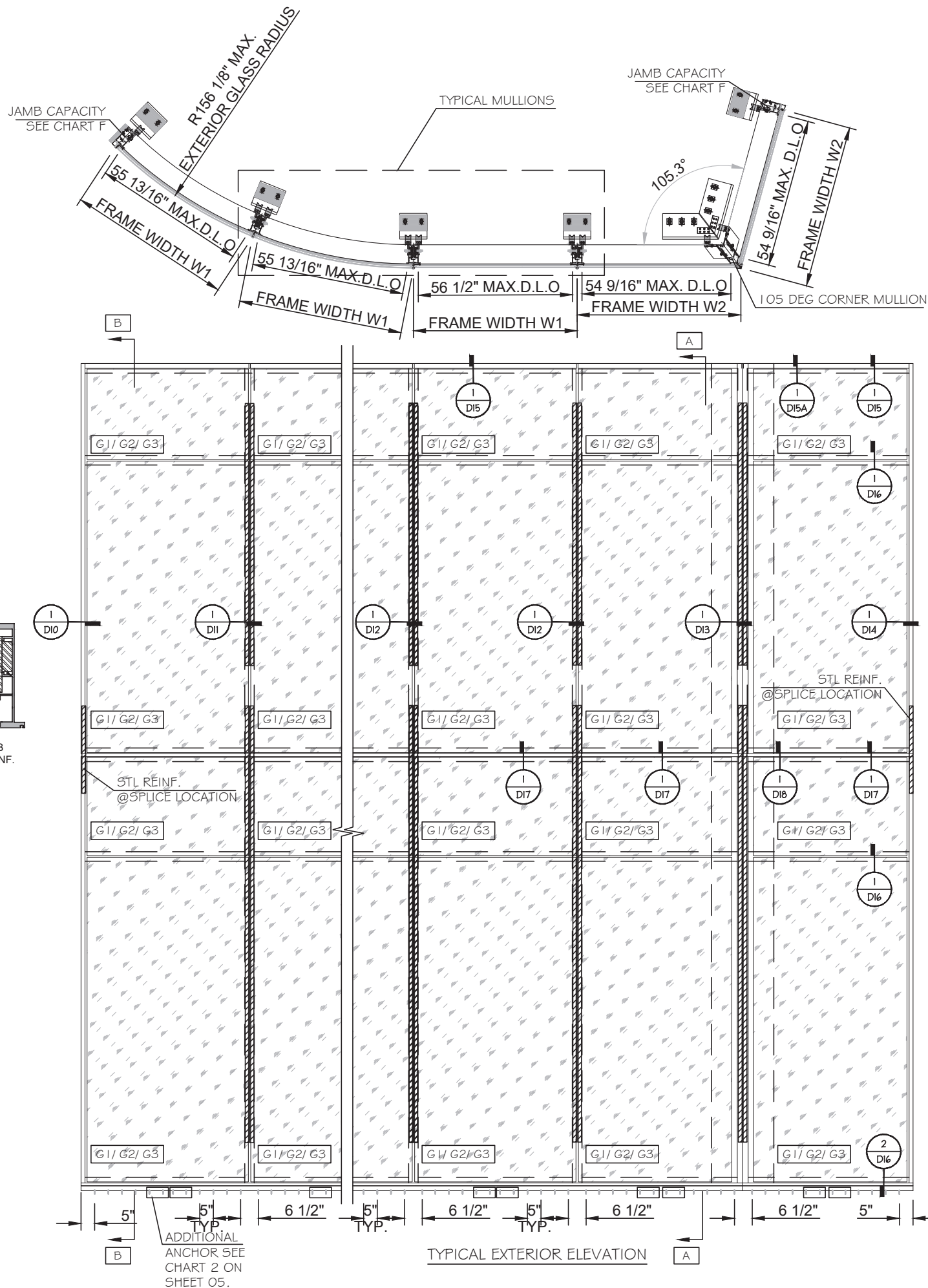
105 DEG CORNER MULLION DESIGN LOAD FRAME WIDTH W=W2 (INCH) REINF. Pd(Psf) 60 W/O +/- 121.6 60 W/ +150/-164 36 W/O +150/-200 50 W/ +150/-200
