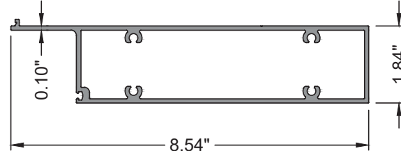
E35 GW-7000-150 HORIZONTAL RAILING ALUM. 6063-T6
