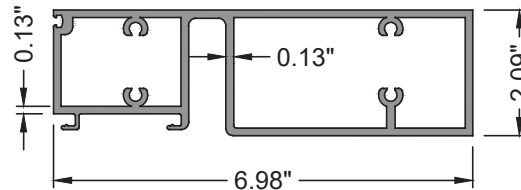
GW-7000-155 SILL ALUM. 6063-T6
