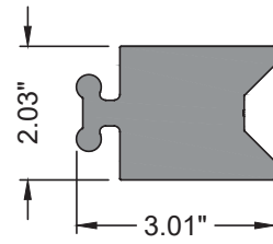
GW-7000-141 MULLION ANCHOR HOOK ALUM. 6061-T6
