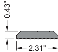
GW-7000-140 SERRATE WASHER ALUM. 6061-T6
