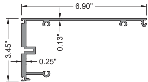
E28 GW-7000-133 HEAD BUTT GLAZED ALUM. 6063-T6
