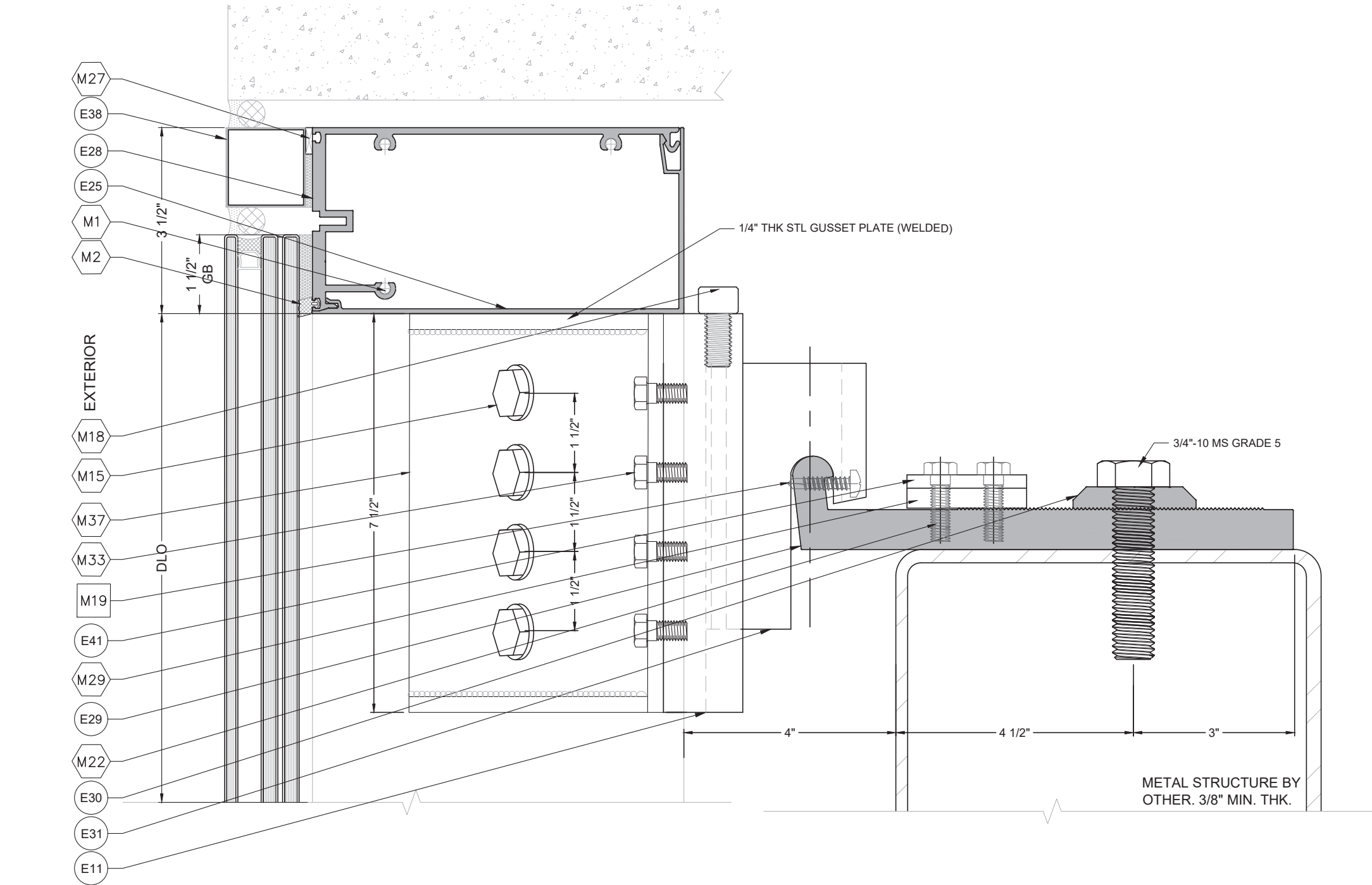
1 DETAIL D15A 105° CORNER MULLION
