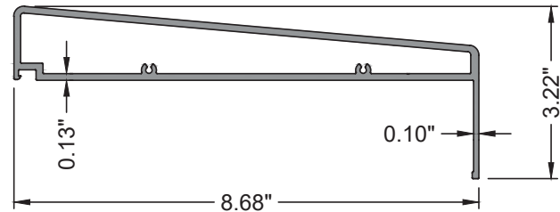
E34 GW-7000-149 RAILING COVER ALUM. 6063-T6
