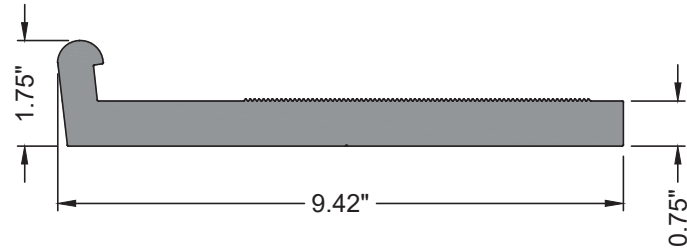
E29 GW-7000-139 SLAB ANCHOR ALUM. 6061-T6
